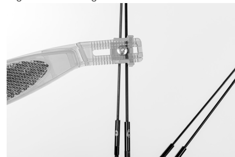
Figure 60: Fitting the side reflectors
